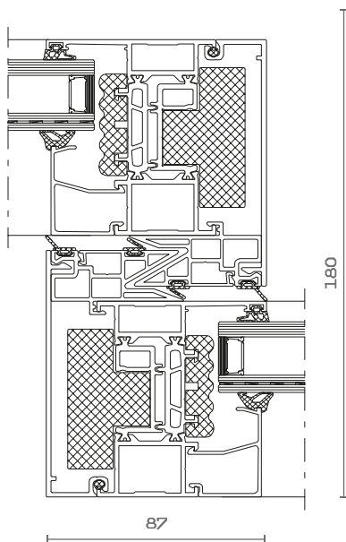
CHICANE
