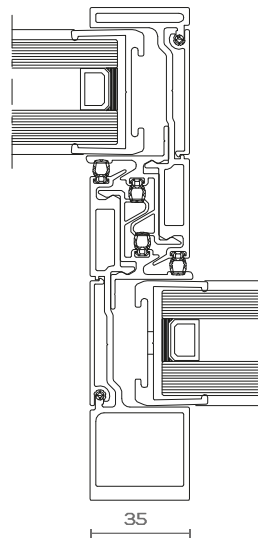
CHICANE
