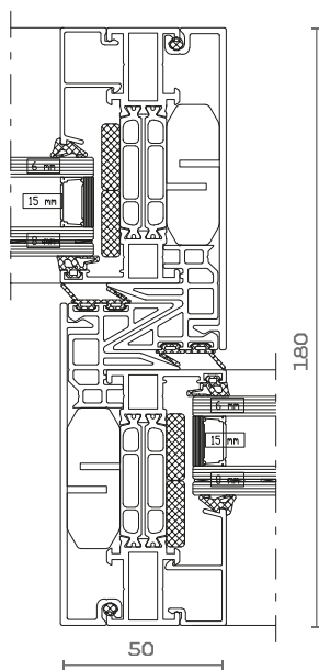
SLIM CHICANE
